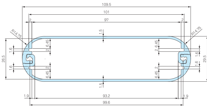
MXFC114-36-□ MXAC/MXC110-30-□
