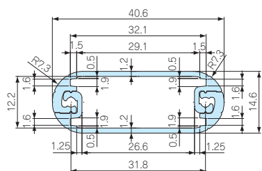
MXAC/MXC41-15-□
