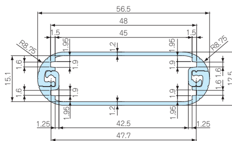
MXFC61-23-□ MXAC/MXC57-18-□
